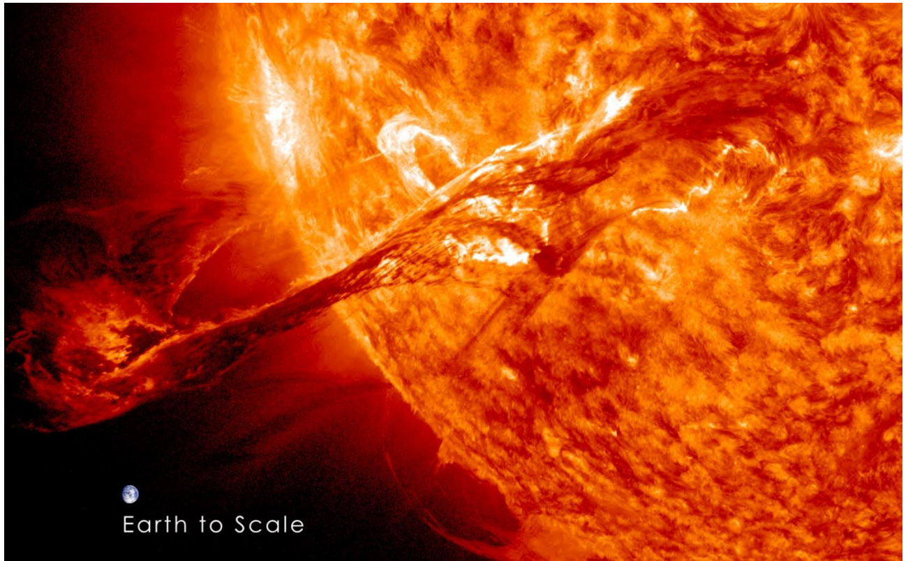
Figure 1 Example of a solar flare
