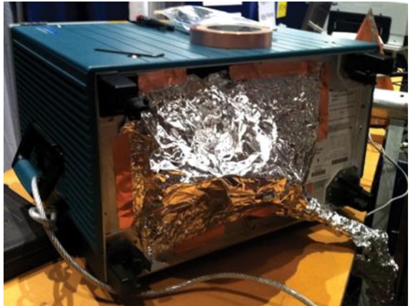
Figure 3: Makeshift Shield to Prevent ESD Induced Measurement Error
